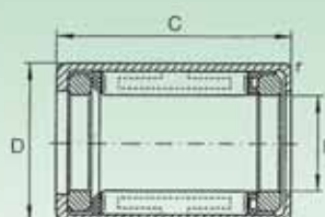
HFL, HFL..KF con cuscinetto strisciante HFL, HFL..KF with plain bearing
