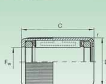
HFL 04 08 KFR HFL 06 15 KFR con zigrinatura with additional knurling
